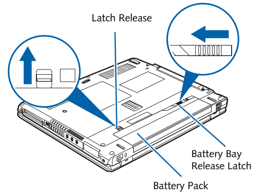
Figure 4-4. Removing a Battery
